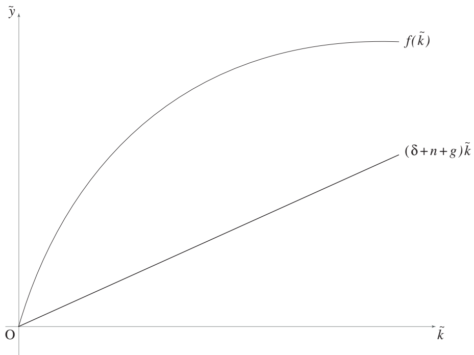
Figure 1: Golden rule steady state
